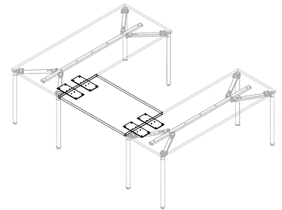
Bridge for U-Shape Desking Supports Bridge Tops 36" - 60" wide
