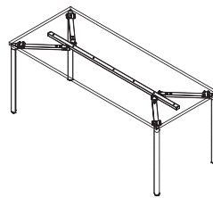
Base + Long Stretcher Bar Supports Tops 72" wide
